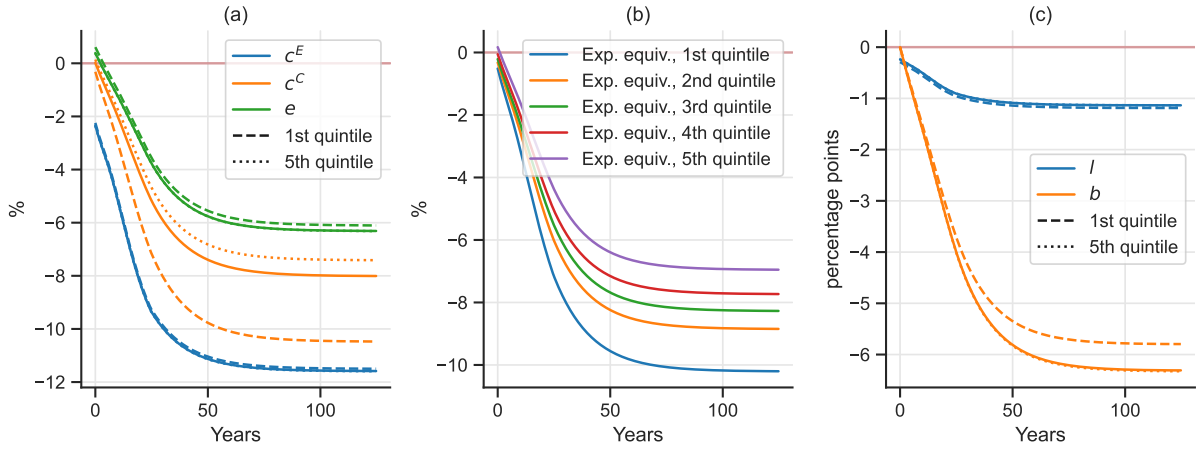
Figure 3: Transition path for consumption, expenditures, expenditure equivalent, labour supply as well as the wealth shares.
